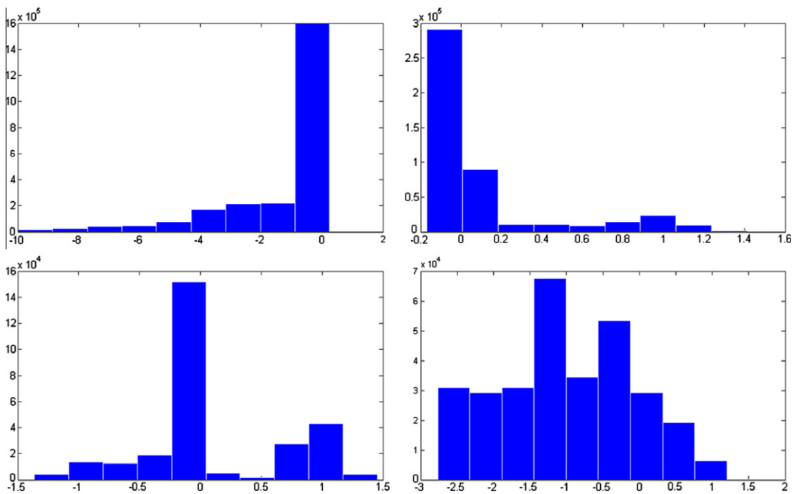
Fig. 11. The histograms of corresponding 3D points to the closest extracted dominant plane in Fig. 10. Noisy points are comparable to points supporting the dominant plane, or even more than the points supporting the dominant plane.
