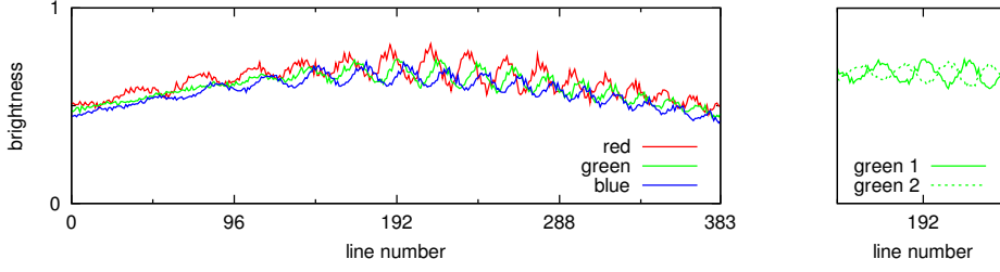
Fig. 1. Left: Brightness levels of the red, green, and blue camera image elements in one column when capturing a red, green, or blue screen, respectively. The Moiré effect is visible in the low amplitude waves, while the base curve shows the general angle dependent light perception. A calibrated camera would show lines with constant brightness levels. Right: The center part of the curves of the two green elements illustrates that the phase shift of the aliasing wave depends on the position of the camera target element.
