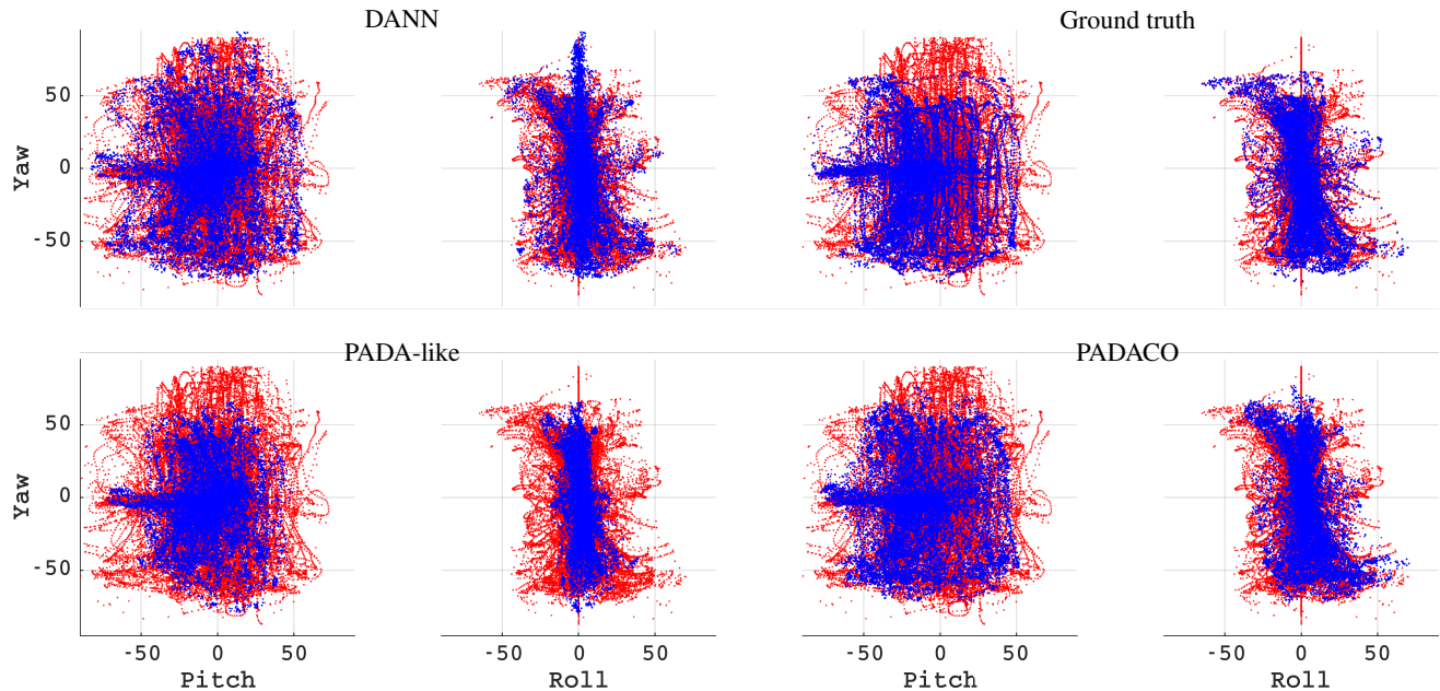
Figure 3. Label space visualization after training with different weighting schemes: In addition to ground truth labels, for every PDA experiment we show source labels Y_s (red) and the predicted target labels \hat{Y}_t (blue). The 3D label space of rotations is visualized by 2D projections on yaw/pitch and yaw/roll (angles in degree). The different distributions reveal the effects of applying the different weighting schemes. DANN [12] expands \hat{Y}_t into Y_s , PADA-like collapses \hat{Y}_t to the higher density regions of Y_s and PADACO (proposed) keeps the overall shape of \hat{Y}_t similar to the ground truth.
