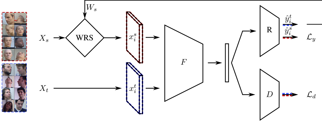
Figure 2. Proposed architecture for domain-adapted head pose estimation: The feature extraction network F is trained to extract domain-invariant features from source and target domain samples ( x_i^s, x_i^t ) using domain-adversarial training. Domain feedback is provided by the domain discriminator D . A pose regressor R estimates the head pose for samples from both domains. Pose estimates from target samples \hat{y}_i^t are feed back to generate sampling weights W_s . Instead of sampling directly from the source data X_s a weighted random sampler (WRS) selects source samples with similar labels to the estimated target labels. This enforces a similar label distribution of source and target domain samples during training.
